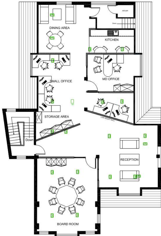
PROPOSED SECOND FLOOR PLAN SCALE 1:50
